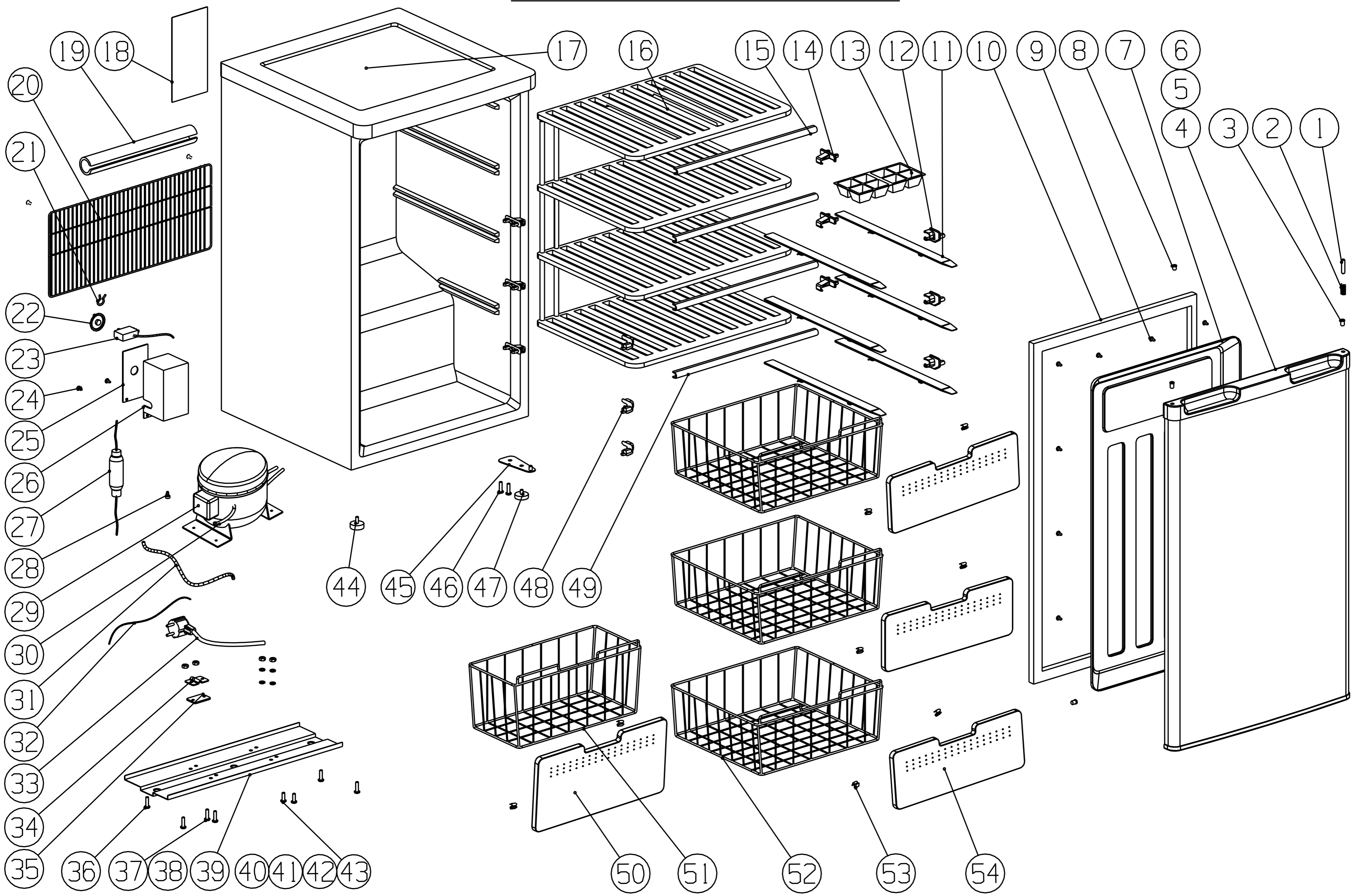
RD-85FA RD-85FB Exploded View
